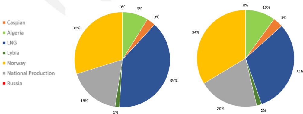
Figure 20 and Figure 21. - Winter RU supply dependence assessment. Reference Winter scenario and sensitivity scenario with low LNG supply potential. Supply mix, %
